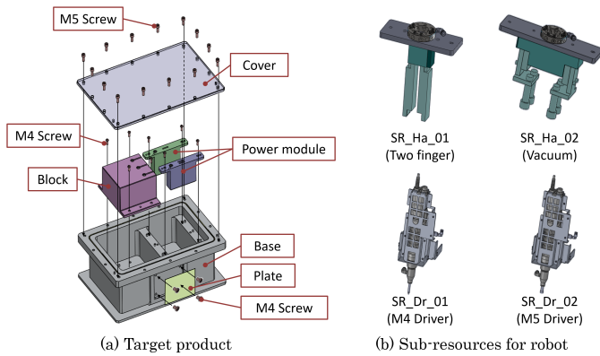
Fig. 1. Product and four robotic tool models in the case study.
